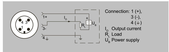
Connection with current output and M12x1 (Ex) device plug
