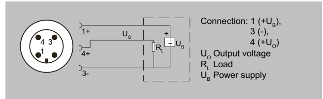
Connection with voltage output, ratiometric output and M12x1 device plug
