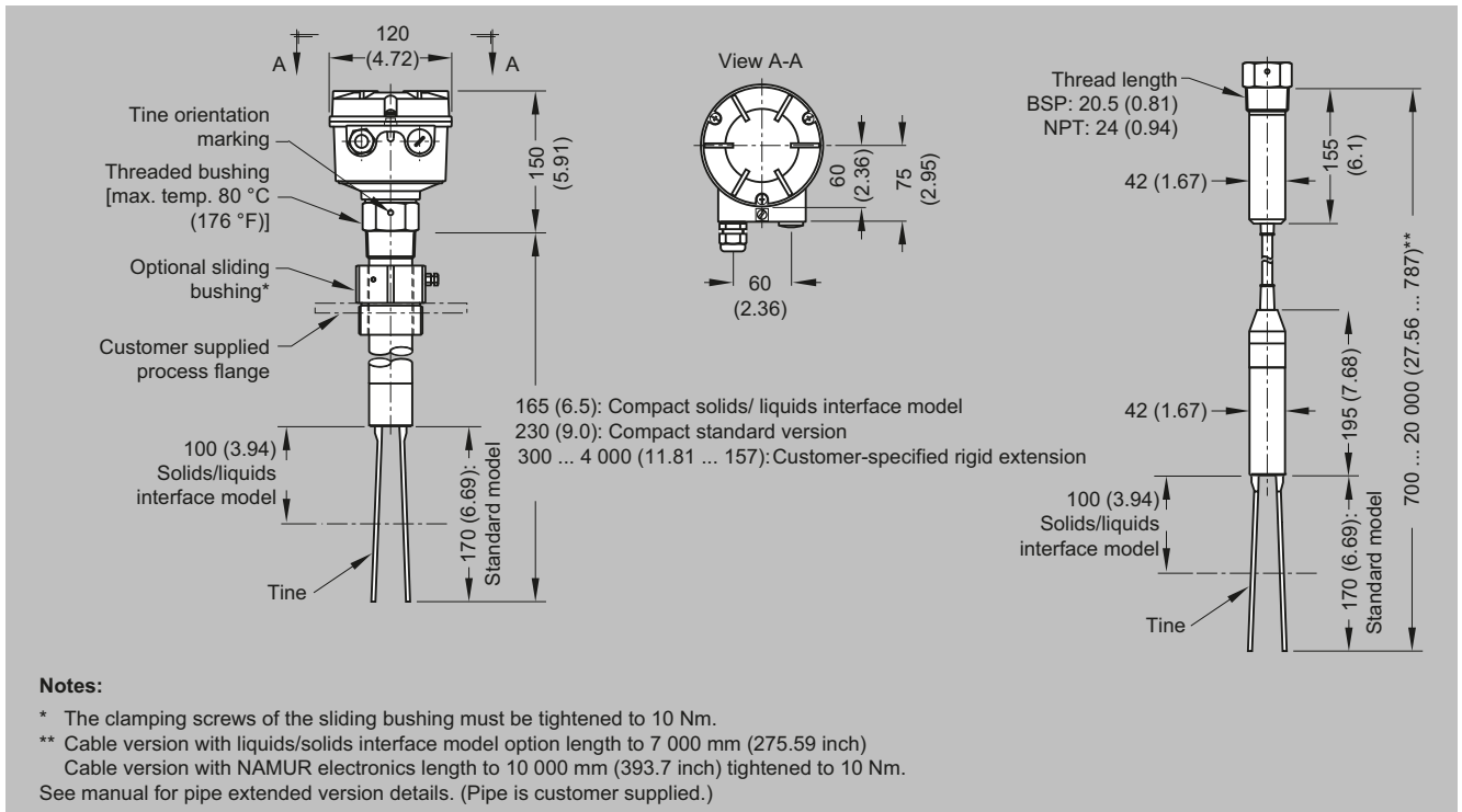
SITRANS LVS200, dimensions in mm (inch)
