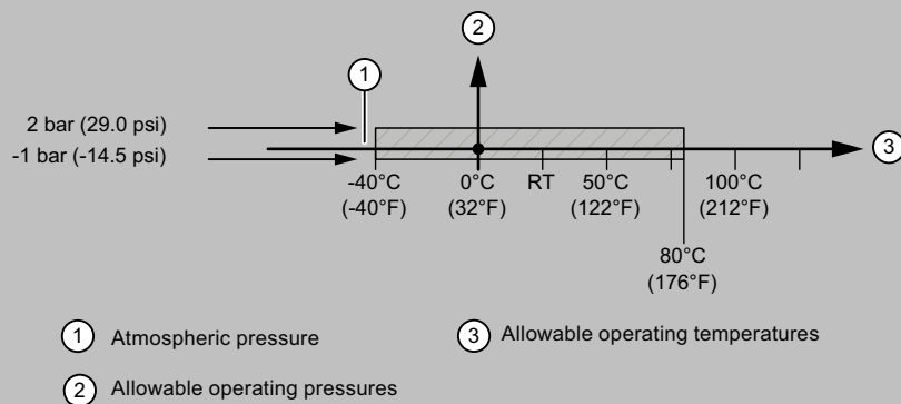
SITRANS LR550 Polymeric horn antenna, process pressure/temperature derating curve
