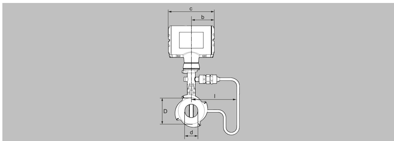
SITRANS FX330 (Vortex), Sandwich version with pressure sensor, side view
