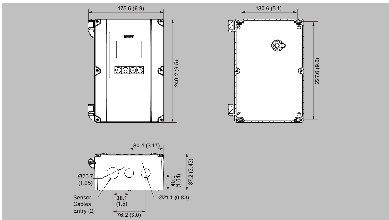
SITRANS FS220 IP65 (NEMA 4X), wall mount enclosure, dimensions in mm (inch)
