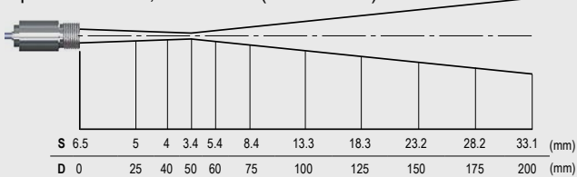
Optics CT LT CF, D:S = 15:1 (far field: 5:1)
