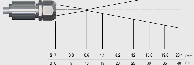
Optics CT LT CF, D:S = 22:1 (far field = 1.5:1)
