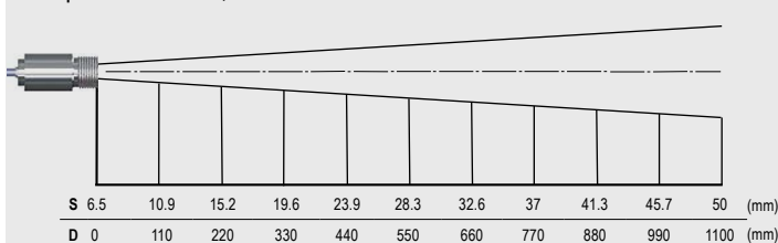
Versions with built-in CF lenses, head length: 32 mm
