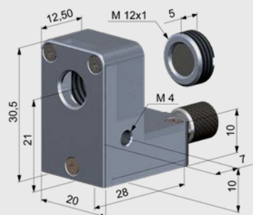
Mounting bracket, fixed (ACCTFB)
