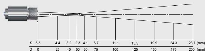
CF optics, D:S = 22:1 (far field = 6:1)
