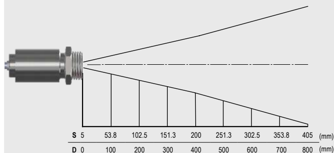
SF optics, D:S = 2:1
