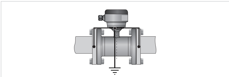
Figure 4-1: Grounding
