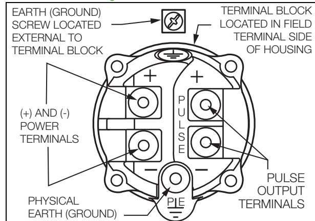
Figure 5. Terminal Block
