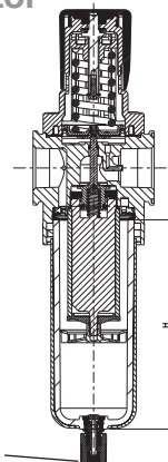
Cross Section - Series 651/652/653 Particulate Filter/ Regulator
