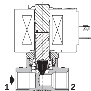
NC function (263 - 3/8)
