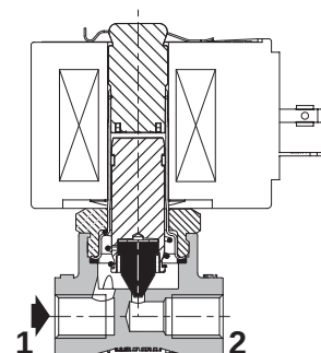
NC function (263 - 1/8)
